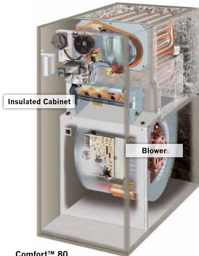
Comfort™ 80 Model 58DLA Gas Furnace shown
